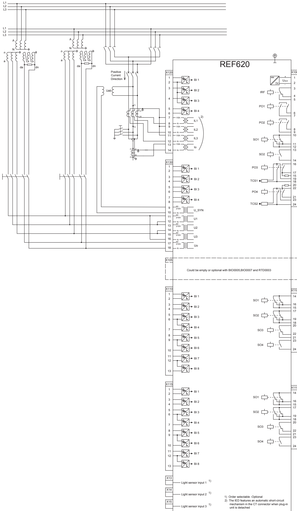
Figure 24. Connection diagram for the configuration with CTs and VTs
