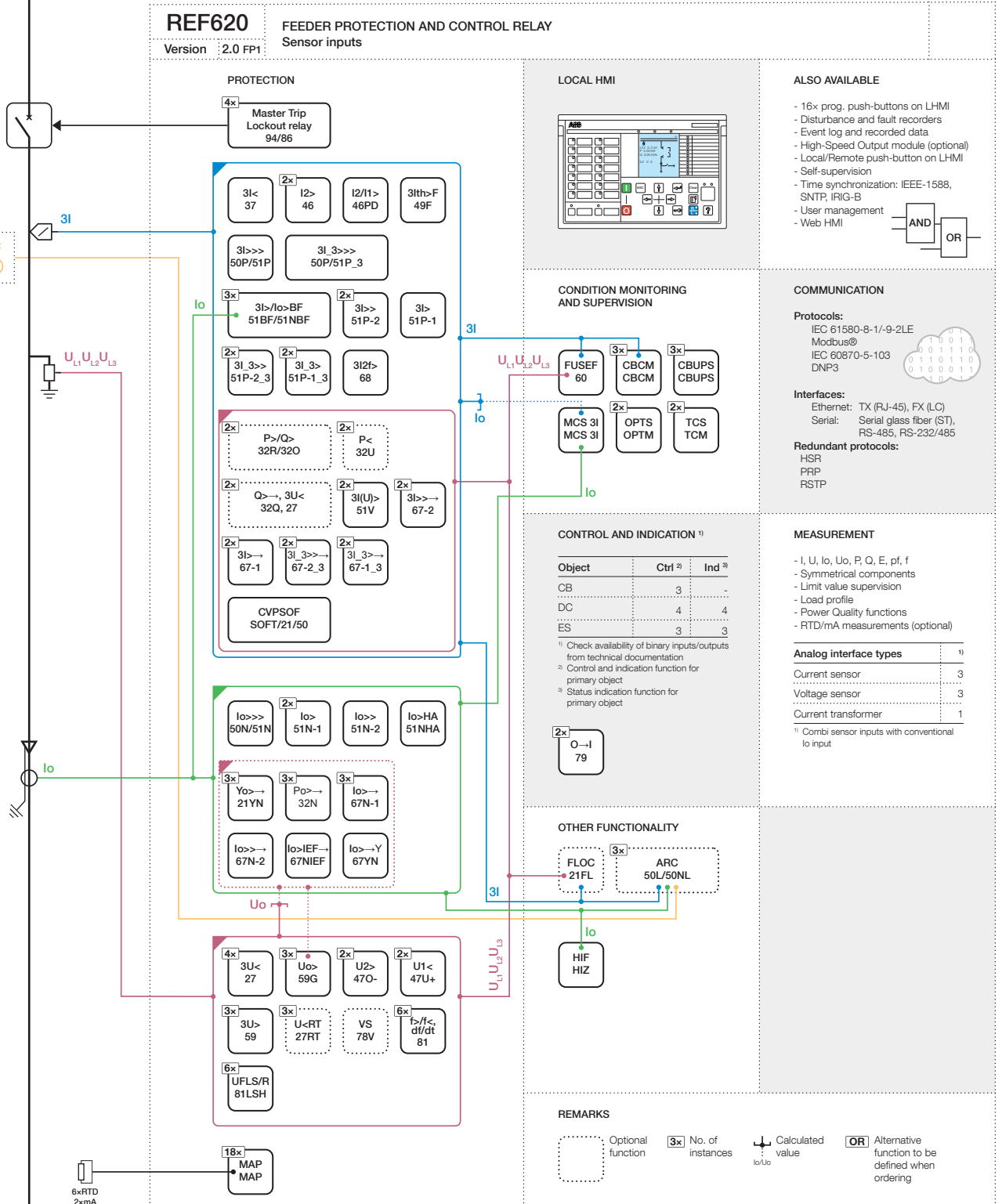
Figure 2. Functionality overview of default configuration with sensor inputs
