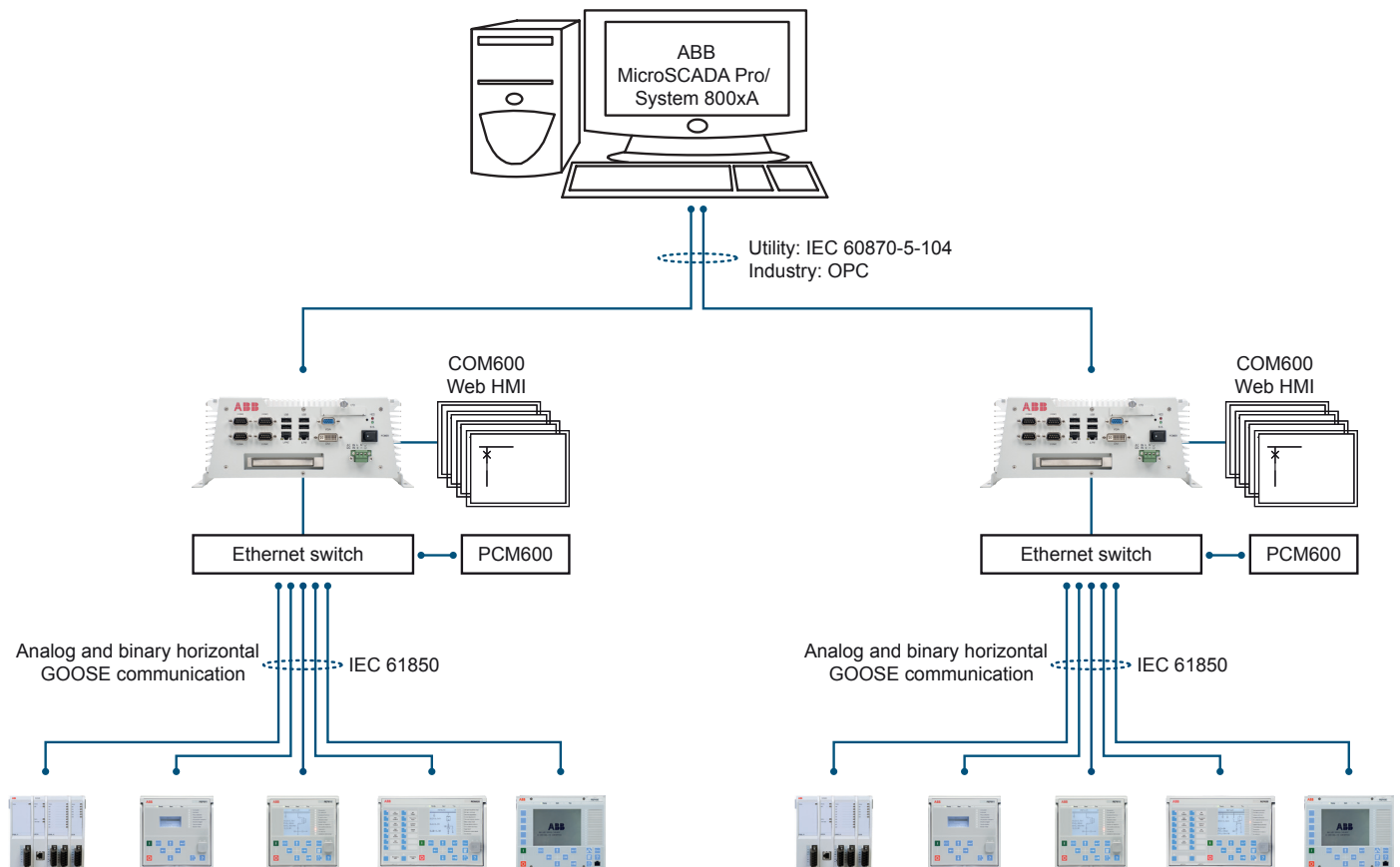
Figure 14. ABB power system example using Relion relays, Substation Management Unit COM600 and MicroSCADA Pro/System 800xA
