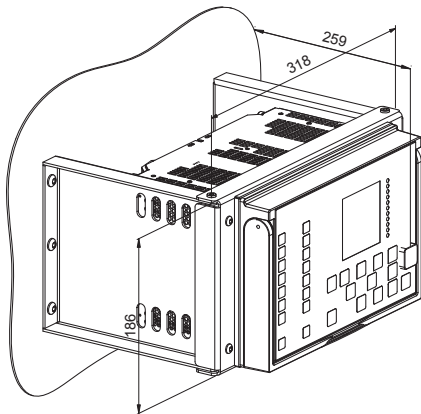
Figure 19. Flush mounting
