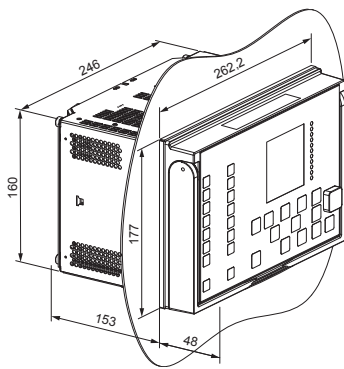
Figure 19. Flush mounting
