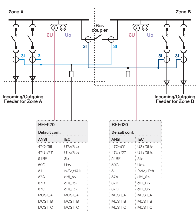
Figure 13. Application example of busbar differential protection covering two zones
