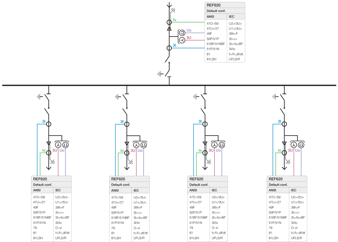
Figure 7. SBB GIS switchgear with the possibility to control the three-position disconnector switch
