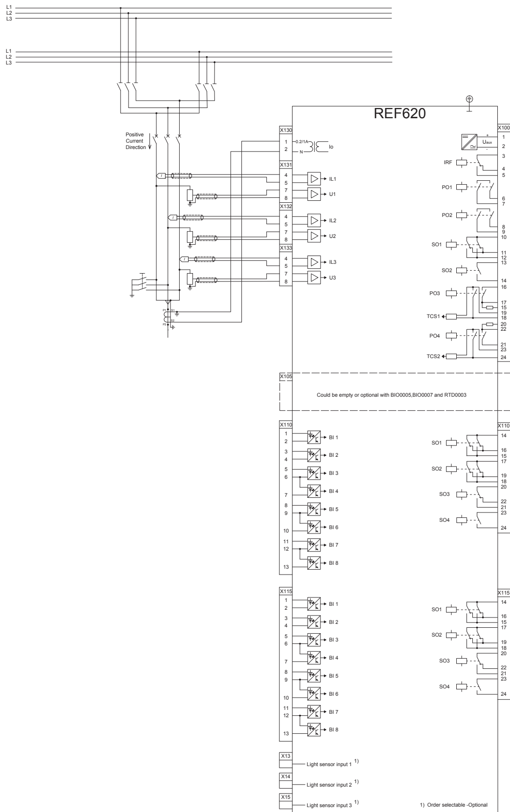
Figure 25. Connection diagram for the configuration with sensors
