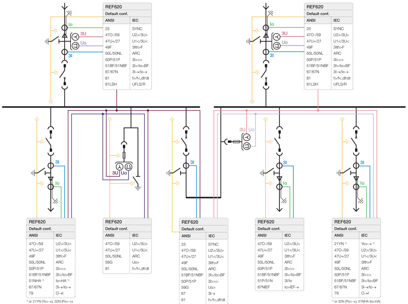
Figure 3. Single busbar AIS 2 section switchgear with conventional instrument transformers
