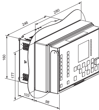
Figure 20. Semi-flush mounting
