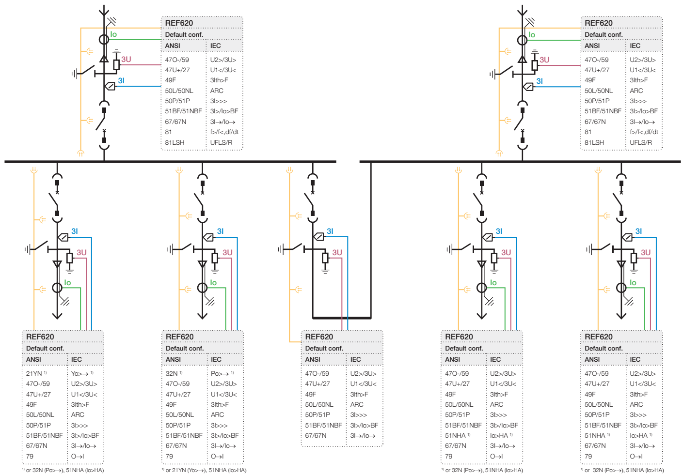
Figure 4. Single busbar AIS switchgear 2 section with sensors
