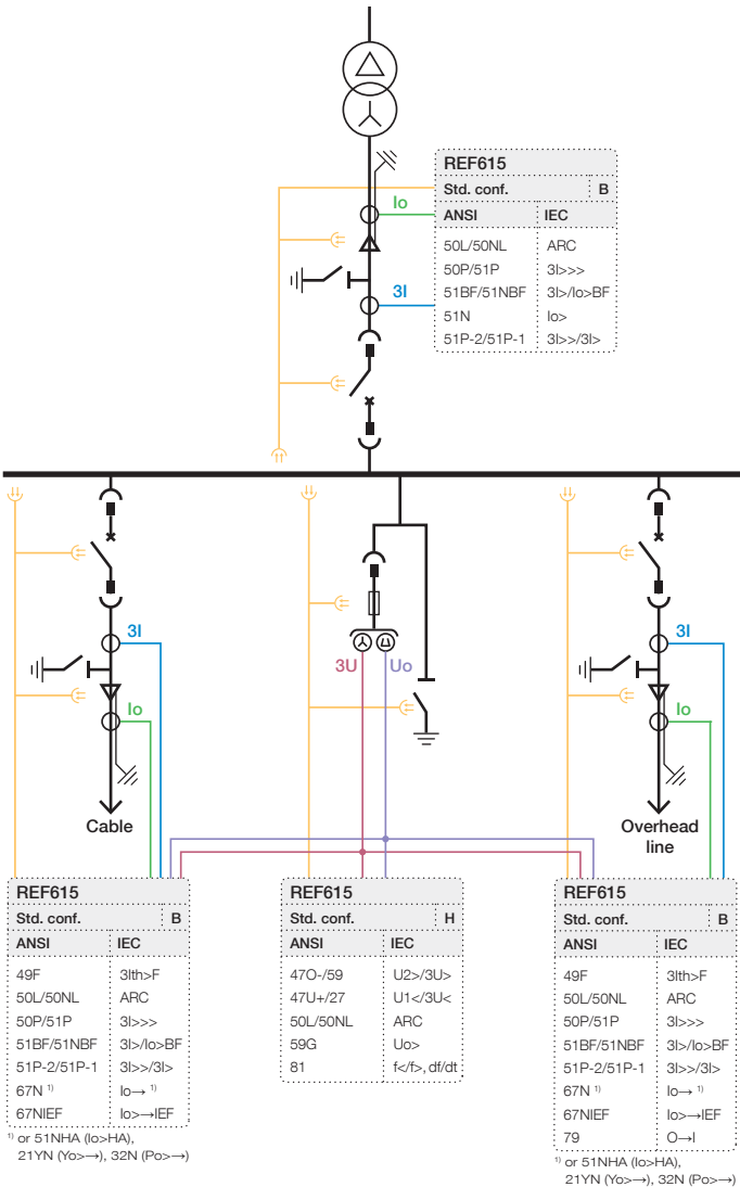
Figure 13. Substation example with overcurrent and earth-fault protection using the standard configuration B
