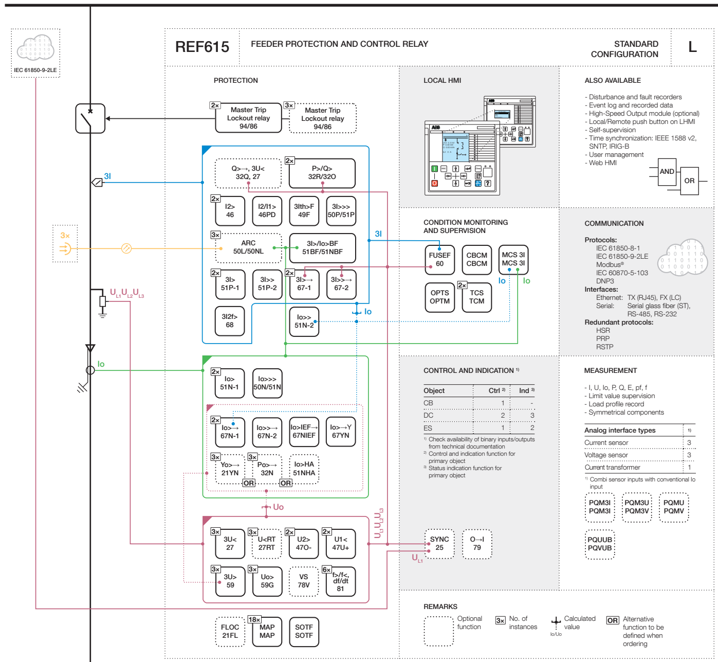
Figure 11. Functionality overview for standard configuration L
