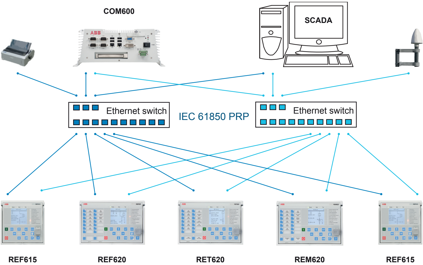
Figure 22. Parallel redundancy protocol (PRP) solution
