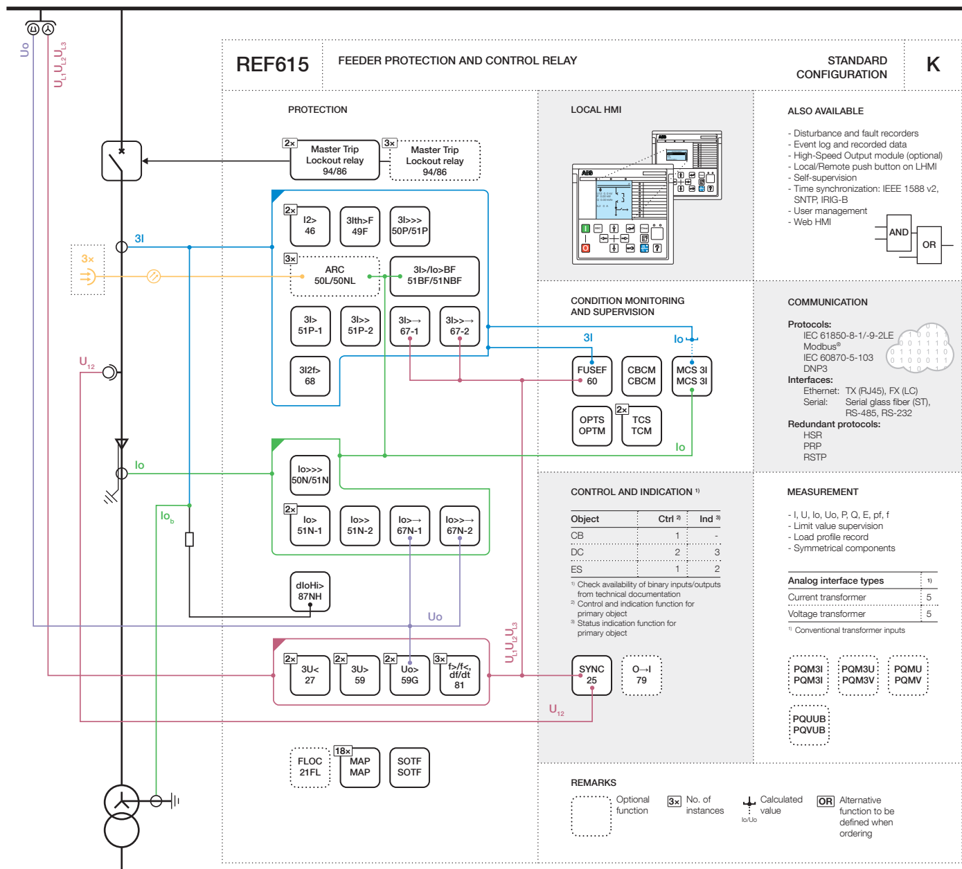
Figure 10. Functionality overview for standard configuration K
