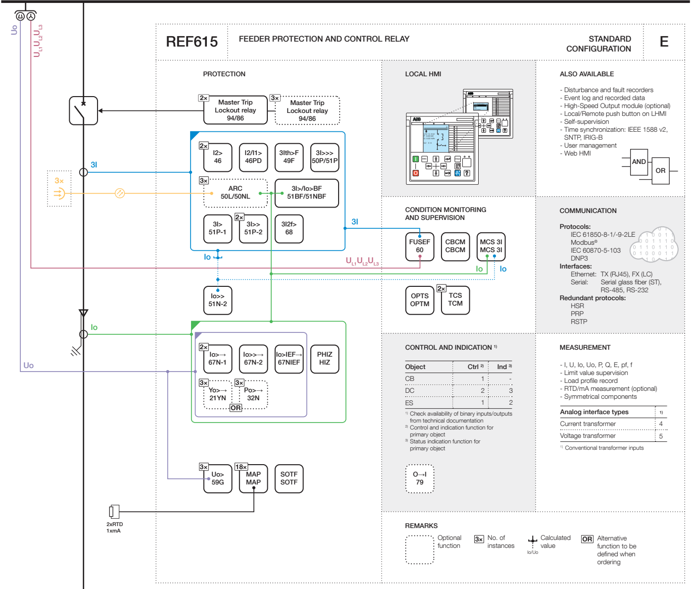
Figure 5. Functionality overview for standard configuration E
