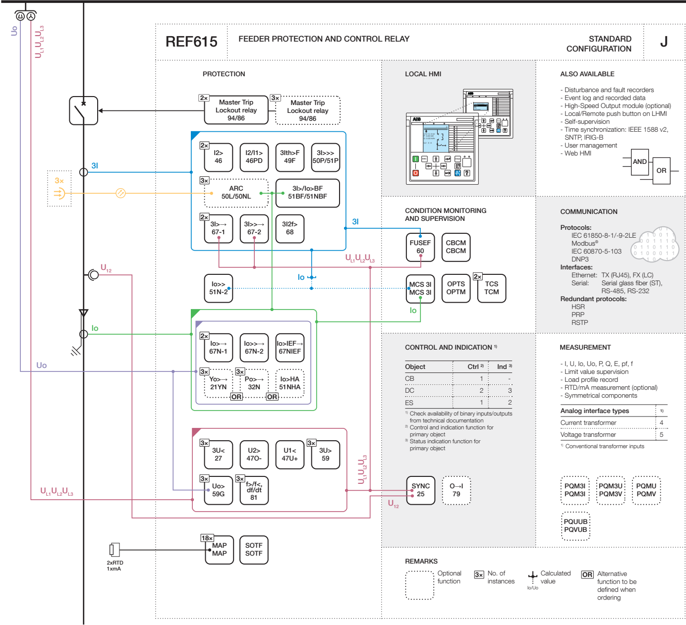
Figure 9. Functionality overview for standard configuration J
